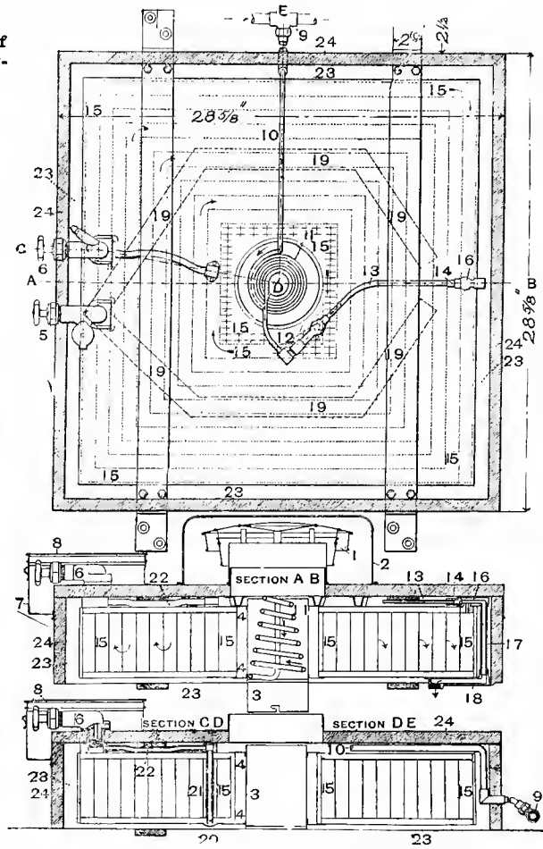
Figs. 3121-3123. Plan and Sections. FROST DRY CARBURETOR.
